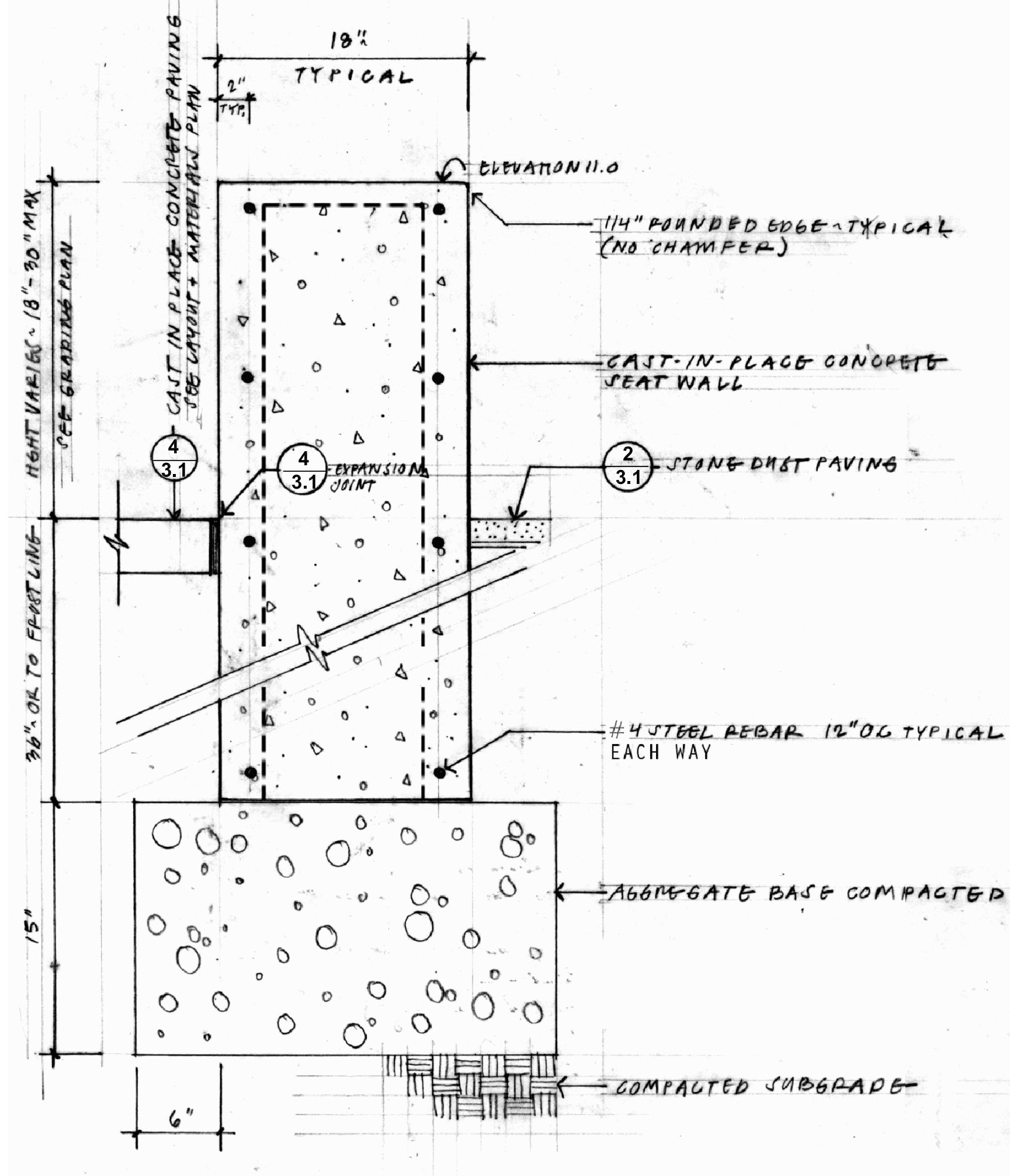
1 Cast in Place Wall : Section Scale: 1-1/2" = 1'-0"
