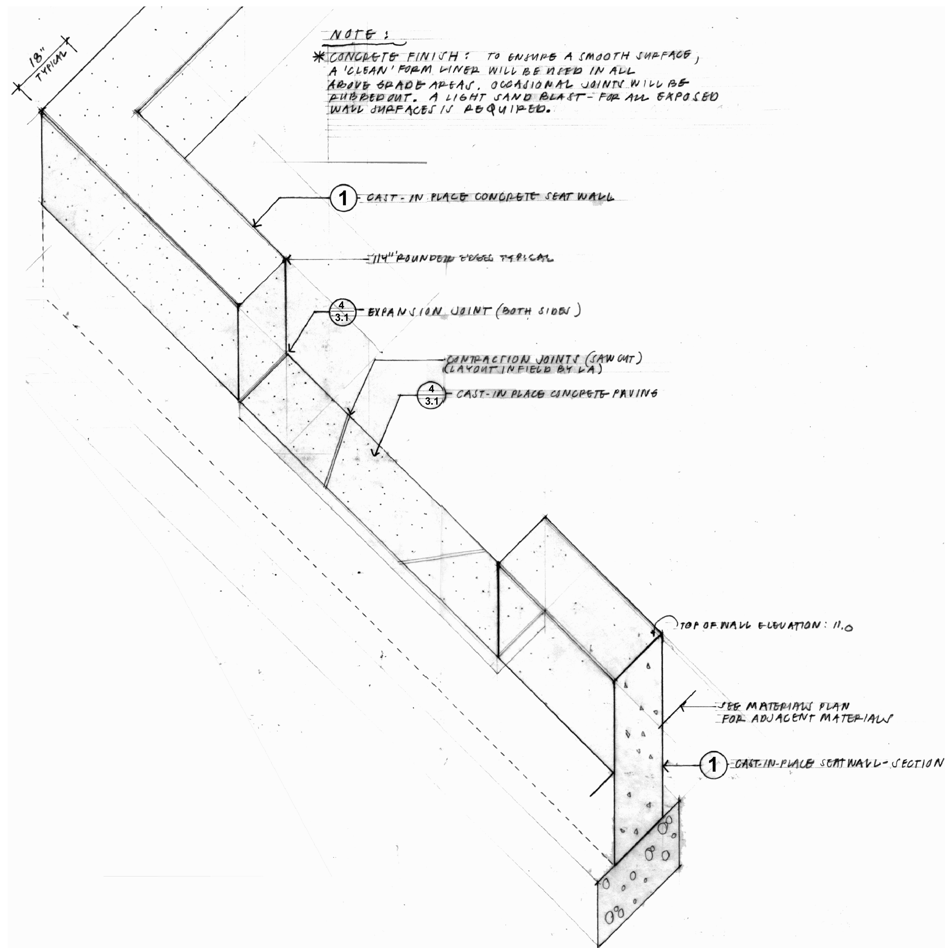
2 Cast in Place Wall : Axon Scale: 3/4" = 1'-0"
