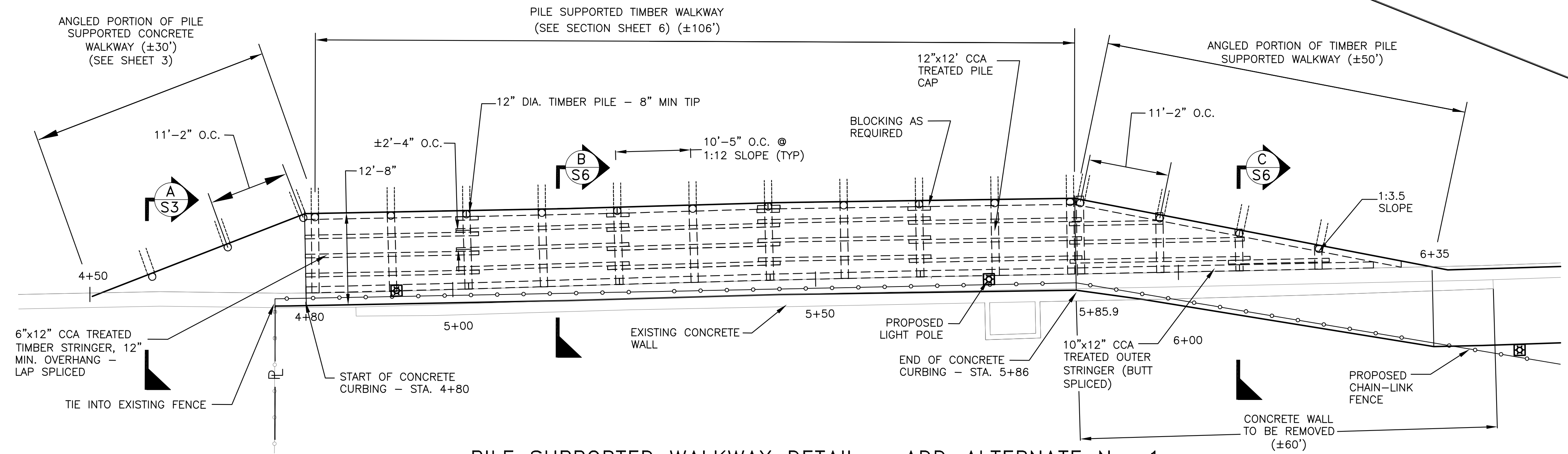
PILE SUPPORTED WALKWAY DETAIL - ADD-ALTERNATE No. 1 SCALE: 1"=10'
