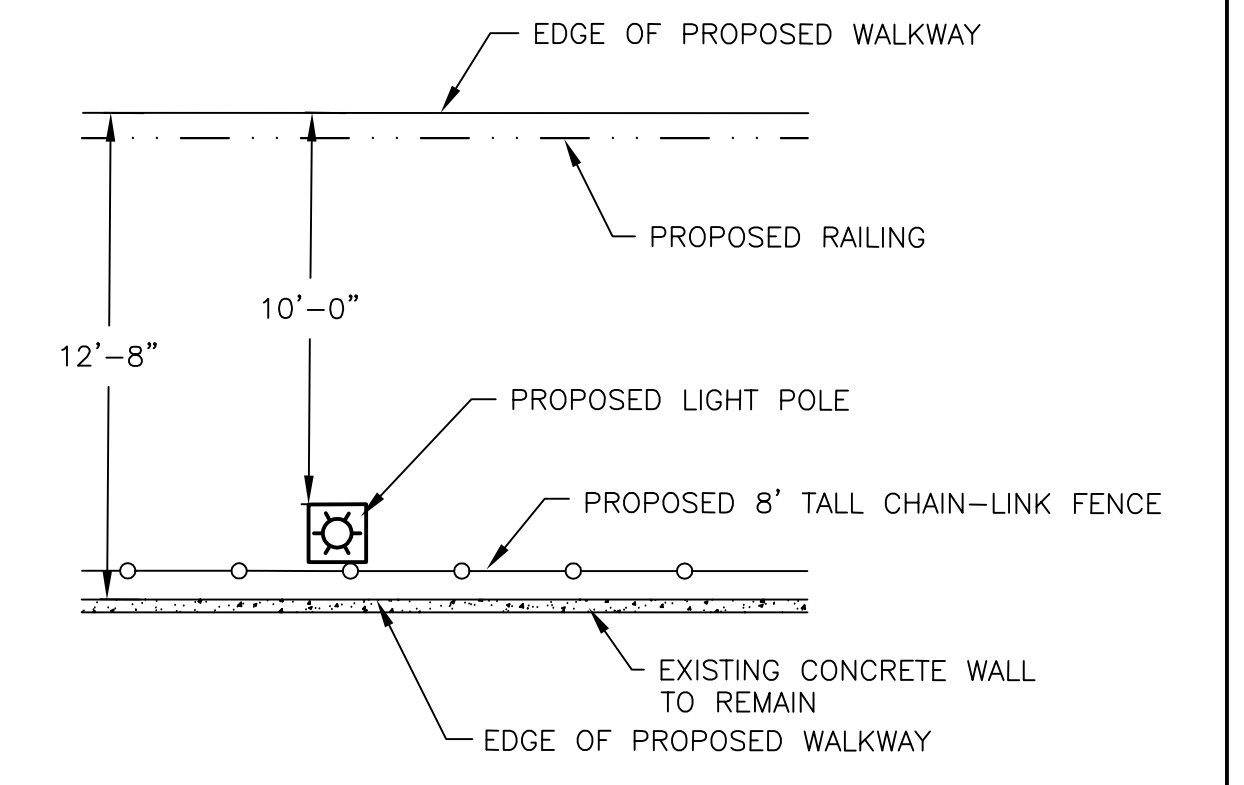
WALKWAY DETAIL - ADD-ALTERNATE No. 1 SCALE: 1"=5'
